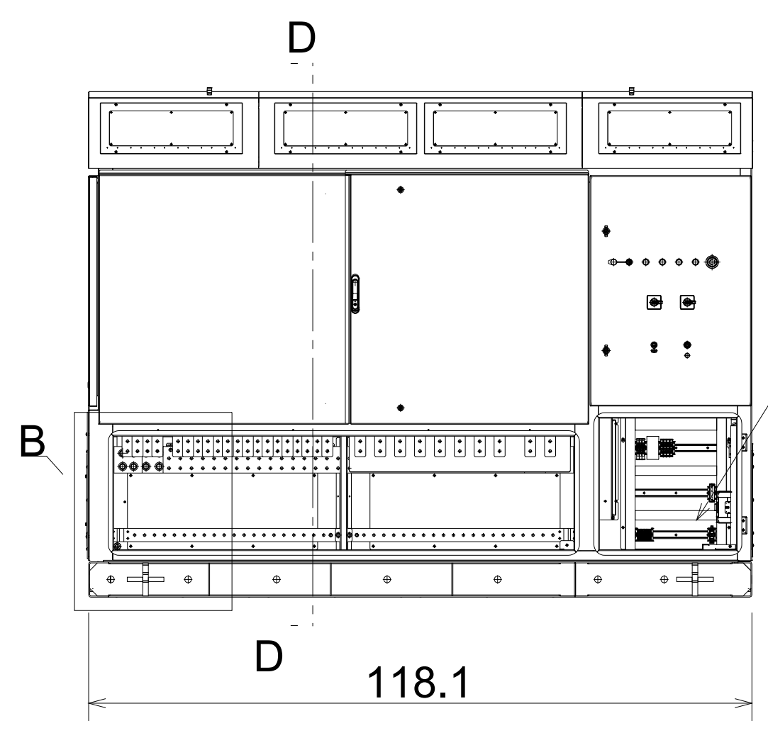
FRONT ELEVATION VIEW (DC UNIT ACCESS)
