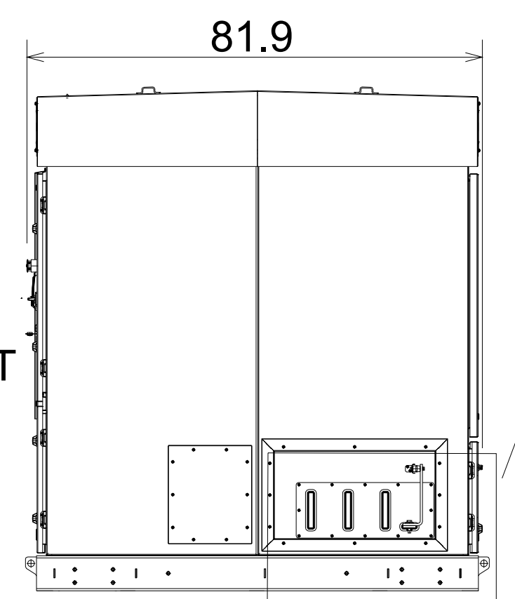
RIGHT SIDE VIEW (AC OUTPUT)
