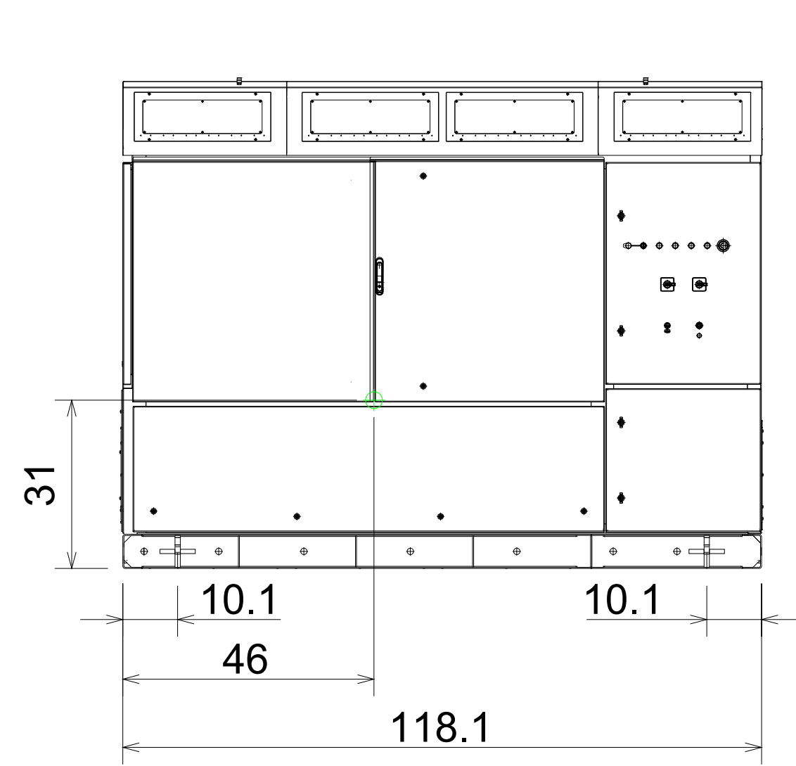
FRONT ELEVATION VIEW (DC UNIT ACCESS)
