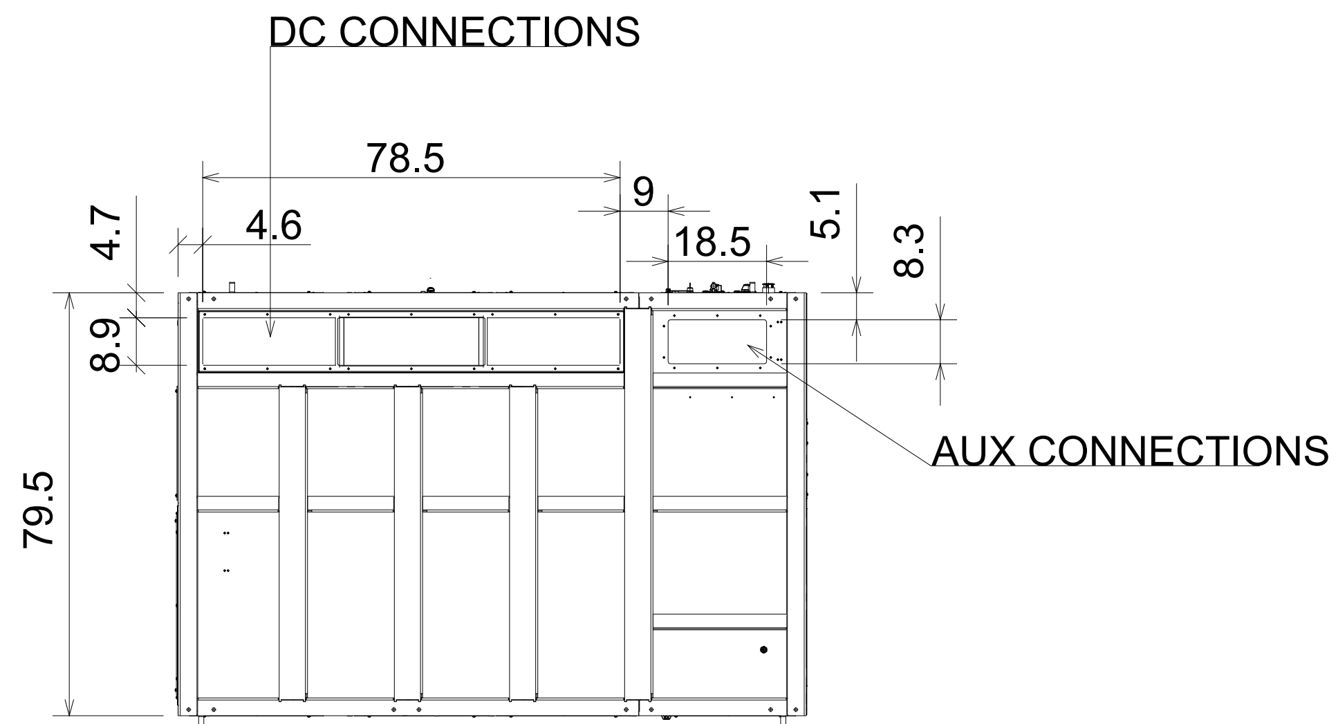
BOTTOM VIEW
