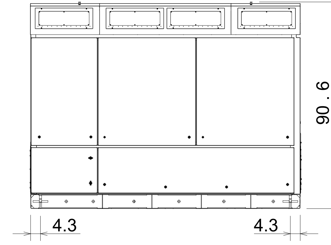
BACK ELEVATION VIEW
