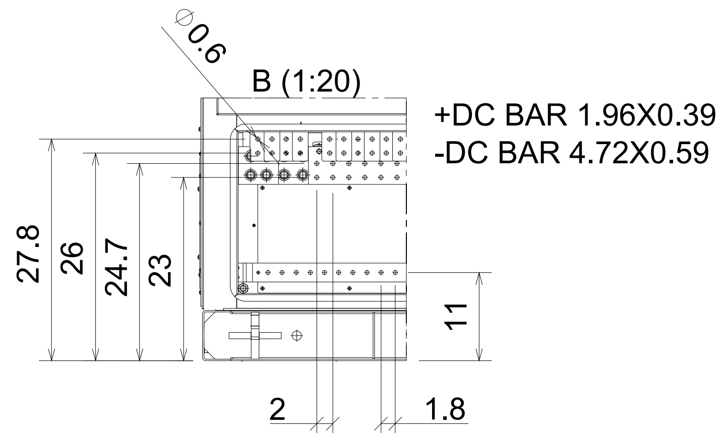
FRONT ELEVATION VIEW (DC UNIT ACCESS)
