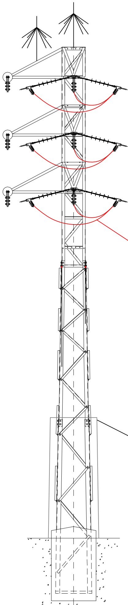
VISTA FRONTAL
